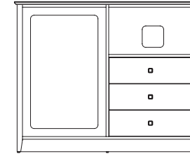
micro/fridge chest left 52" w x 24" d x 42" h microwave opening: 23" w x 21" d x 13" h refrigerator opening: 23" w x 21" d x 36" h 3 drawers with ball bearing glides recessed / vented back 1 fixed shelf high pressure laminate top with solid wood edge
