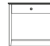
nightstand 24" w x 16" d x 28" h 30" w x 16" d x 28" h 1 drawer with ball bearing glides recessed back 1 fixed shelf high pressure laminate top with solid wood edge
