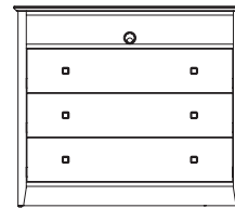
media chest 42" w x 22" d x 36" h media opening: 37.5" w x 19" d x 5.25" h 3 drawers with ball bearing glides recessed / vented back 1 fixed shelf high pressure laminate top with solid wood edge
