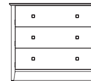
chest 36" w x 22" d x 30" h 3 drawers with ball bearing glides recessed back high pressure laminate top with solid wood edge
