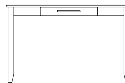
desk with drawer 48" w x 28" d x 30" h 1 drawer with ball bearing glides high pressure laminate top with solid wood edge apron to floor: 26"
